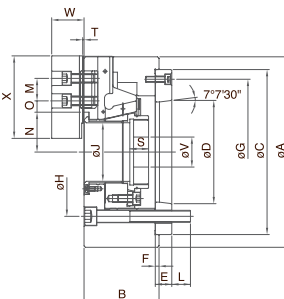
MODEL BBC 3-JAW WEDGE TYPE POWER CHUCK
