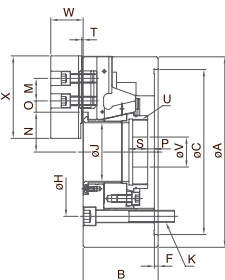
MODEL BBC 3-JAW WEDGE TYPE POWER CHUCK
