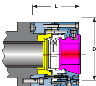
Spindle Style 1
