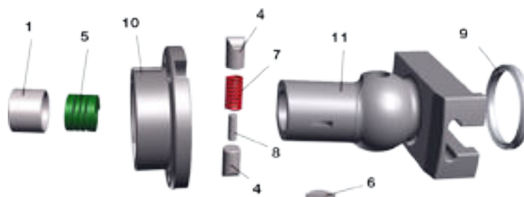
Standard Arm Kit
