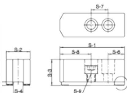
SOFT JAW SPECIFICATIONS
