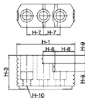
HARD JAW SPECIFICATIONS
